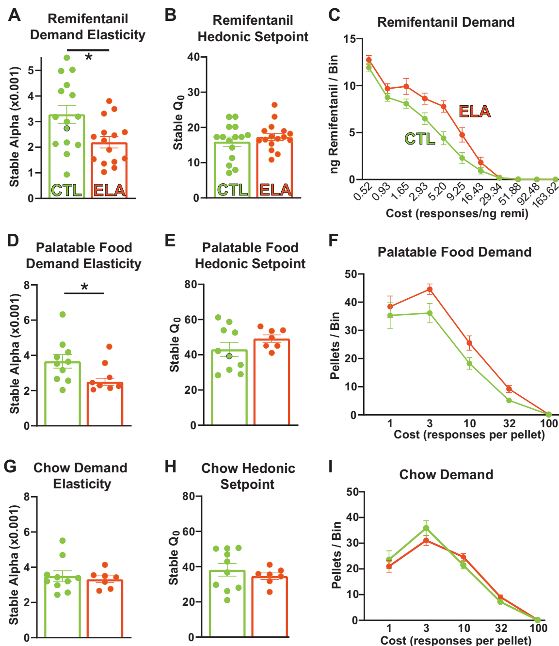
Fig. 2 Early life adversity increases demand for opioids and highly palatable food. a ELA-reared rats had a decreased sensitivity to cost, or an ‘inelastic’ demand, for remifentanyl compared with controls ( t_{28} = 2.630 ; P = 0.0137 ). b However, no changes were observed in the intake of remifentanyl by the ELA group when the drug was essentially “free”, measured as the hedonic set-point, or Q_0 ( t_{28} = 0.8159 ; P = 0.4215 ). c Average ( \pm SEM) drug intake at each effort step is depicted. d ELA rats were willing to pay a significantly higher price (effort) for a highly palatable food, indicating decreased demand elasticity, or \alpha ( t_{15} = 2.341 , P = 0.0334 ), whereas (e) consumption at
